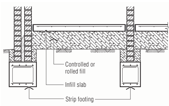
Figure 7.5 Strip footing
