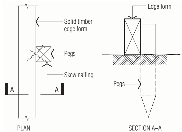
Figure 5.1 Basic ground forms
