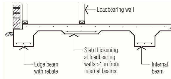
Figure 7.1 Stiffened raft
