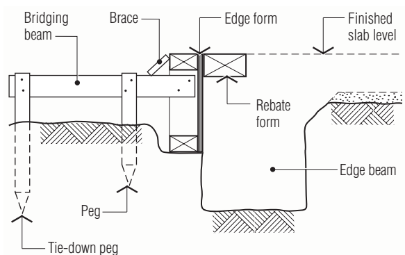
Figure 5.4 Formwork for raft slab with rebate
