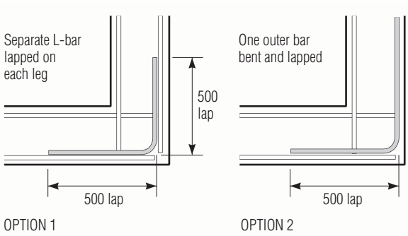
Figure 5.12 Lapping of reinforcement at corners
