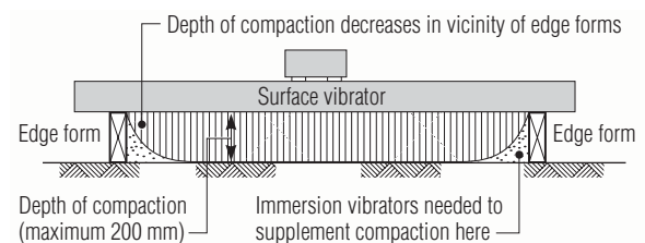
Figure 4.7 Degree of compaction varies across width when surface vibrators are supported off edge forms
