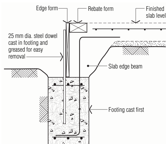
Figure 5.6 Formwork for footing slab
