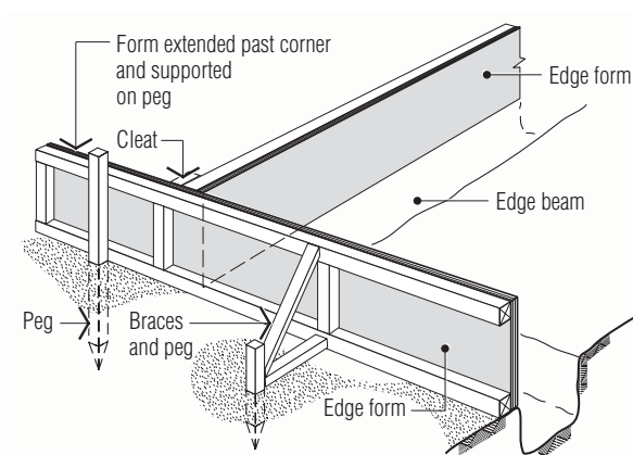
(a) CARRY ONE EDGE FORM PAST THE CORNER
