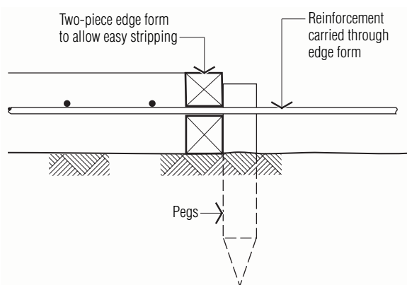
(a) TWO-PIECE FORMWORK TO ALLOW REINFORCEMENT CONTINUITY
