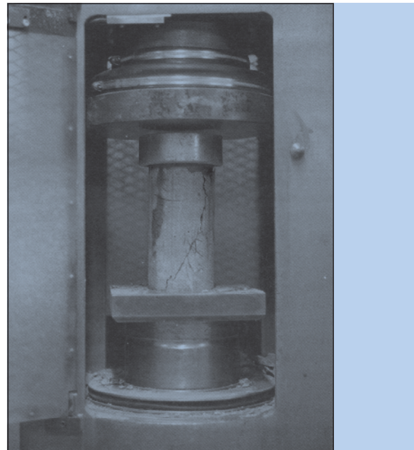
Figure 3.5 Compression testing of concrete cylinder
