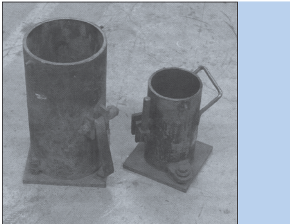
Figure 3.4 100 and 150-mm-diameter compression test cylinder moulds
