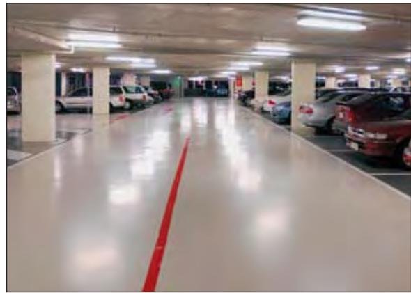
Figure 9.7 Coating used in garage area to provide uniform colour, delineate areas, protect surface and facilitate cleaning
