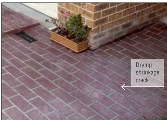
Figure 6.6 Drying shrinkage crack caused by restraint of brick wall
