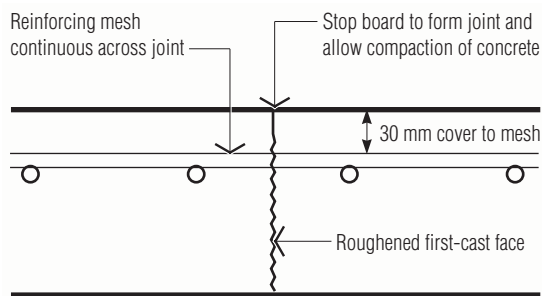
Figure 6.13 Typical construction joint detail
