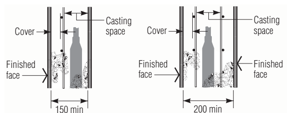
Figure 4.5 Provide sufficient clearances to allow compaction
