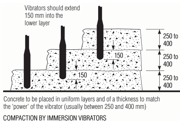
Figure 4.3 Compaction of concrete placed in layers
