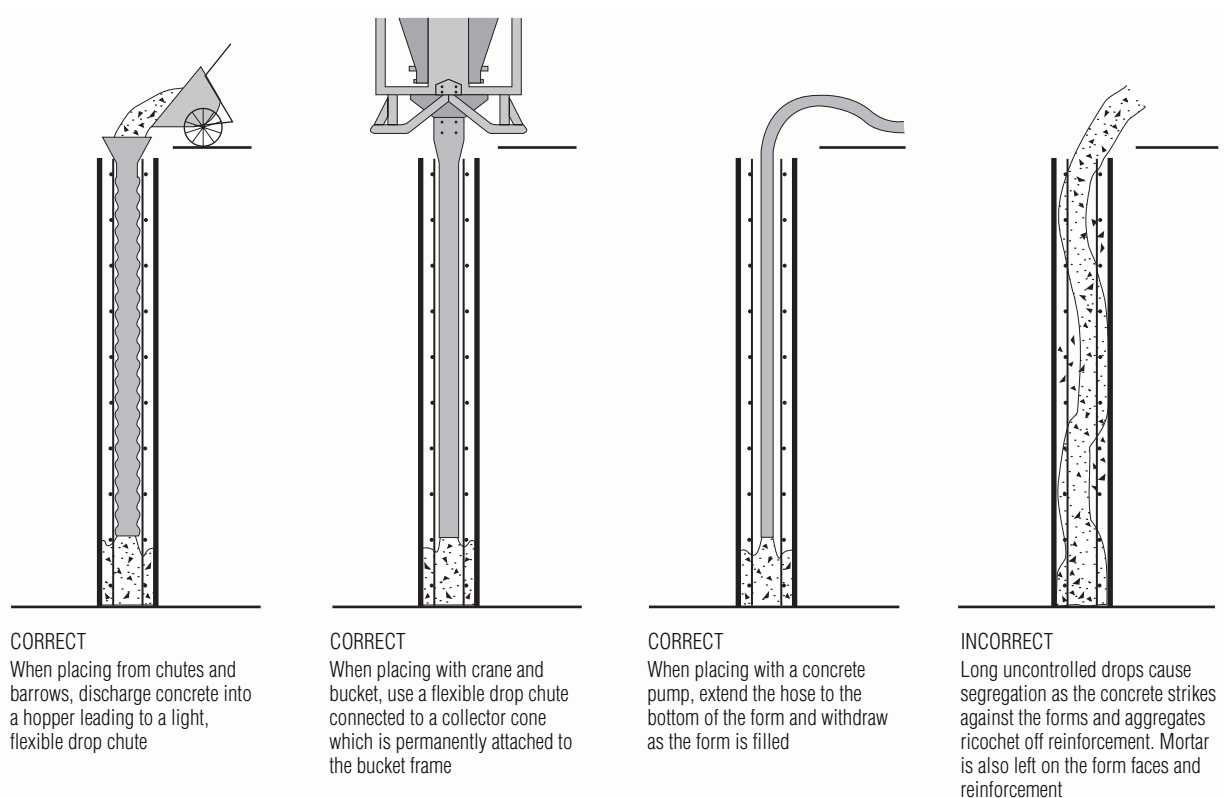
Figure 4.2 Placing techniques for walls and columns
