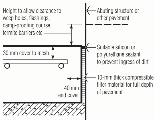
Figure 6.7 Typical isolation joint detail
