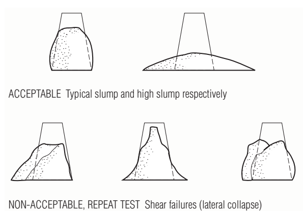
Figure 3.3 Examples of slump
