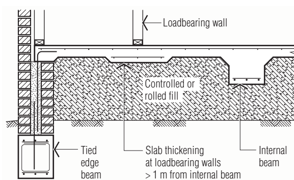
Figure 7.3 Stiffened slab with deep edge beam
