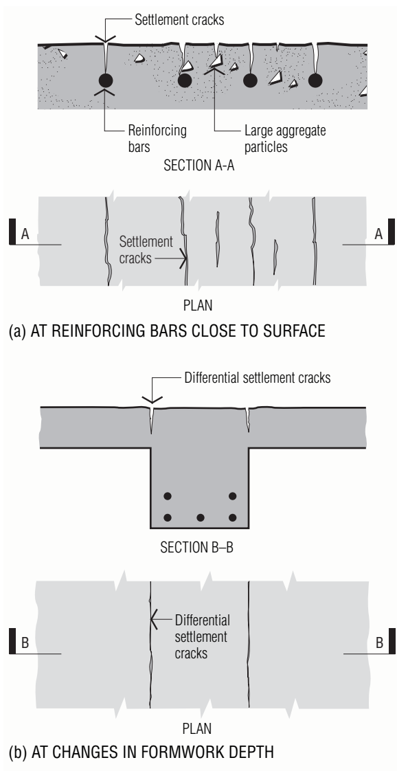
Figure 6.2 Plastic settlement cracking
