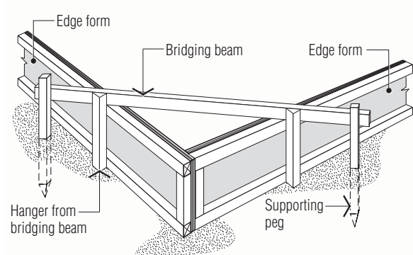
(b) HANG EDGE FORMS FROM A BRIDGING BEAM
