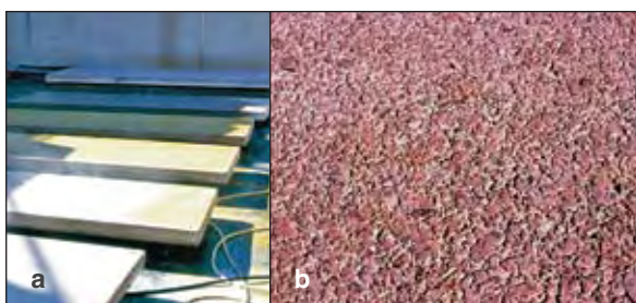
Figure 9.19 (a) Acid etching process and (b) close-up of heavy etching
