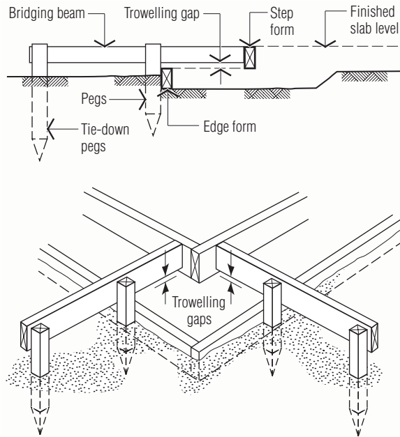
Figure 5.7 Cantilevered formwork
