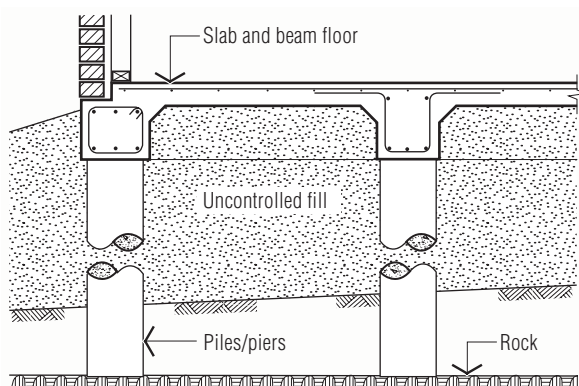
Figure 7.6 Pier/pile and slab footing
