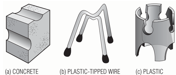
Figure 5.11 Typical spacers for reinforcement
