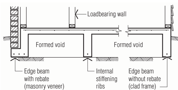
Figure 7.2 Waffle raft
