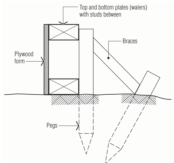
Figure 5.2 Braced formwork for slabs more than 150 mm thick
