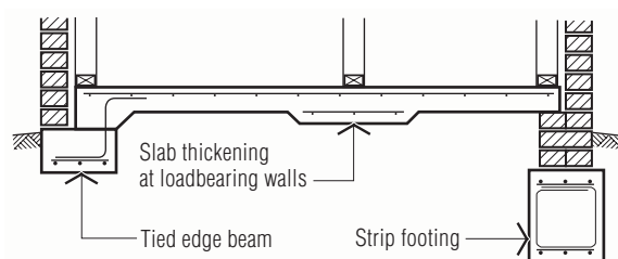
Figure 7.4 Footing slab
