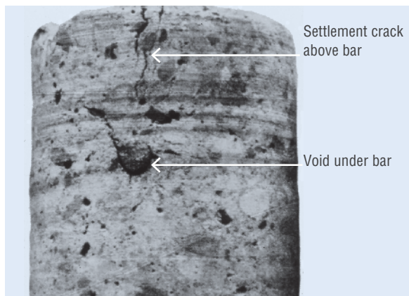
Figure 6.3 Plastic settlement crack above reinforcing bar with void under bar
