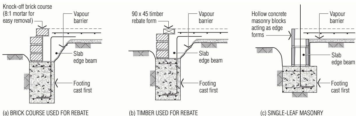
Figure 5.8 Masonry formwork
