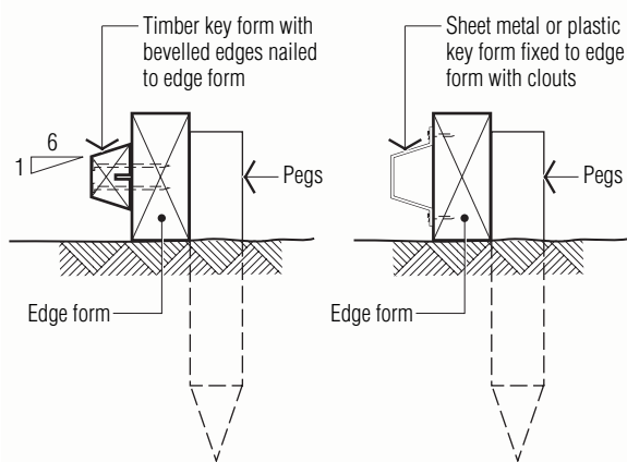
(b) TIMBER, METAL AND PLASTIC KEY JOINTS
