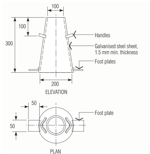
Figure 3.1 Typical cone for slump test
