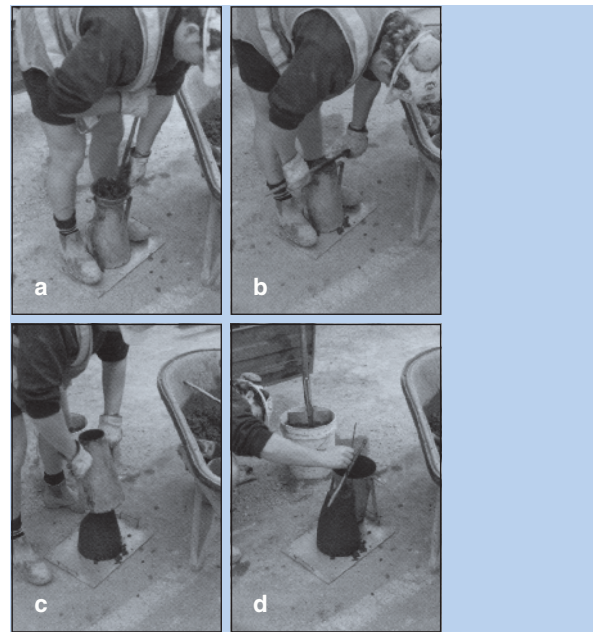
Figure 3.2 Slump test
