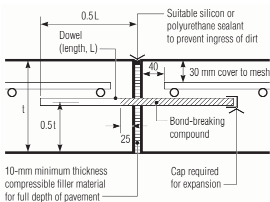
Figure 6.8 Typical expansion joint detail
